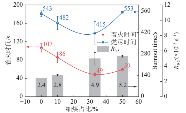
图8 不同细煤占比下混煤工况的燃烧结果 Fig. 8 Combustion of mixed particle coal under different fine coal ratios
