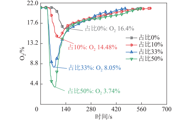
图9 不同细煤占比下混煤工况的 O 2 浓度曲线 Fig. 9 O 2 curves of mixed particle coal combustion under different fine coal ratios
